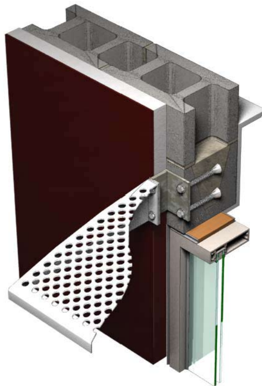
ISOMETRIC RENDERING
