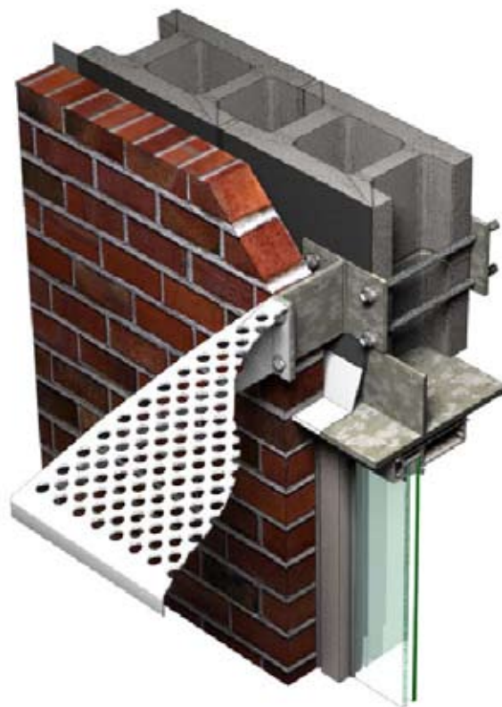
ISOMETRIC RENDERING
