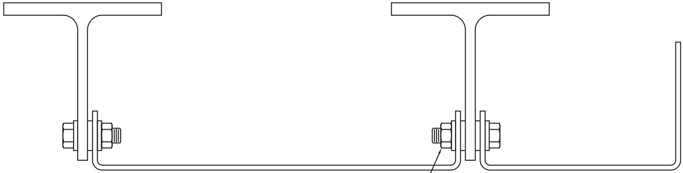
BOLTED CONNECTION WITH WITH SPACER WASHERS
