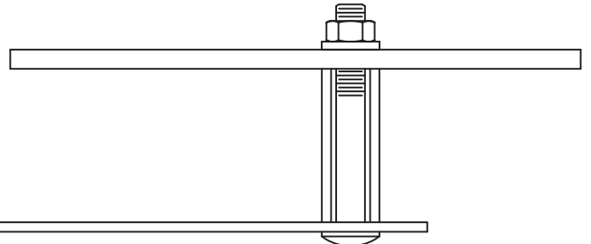
CARRIAGE BOLT WITH TUBE STEEL SPACER
